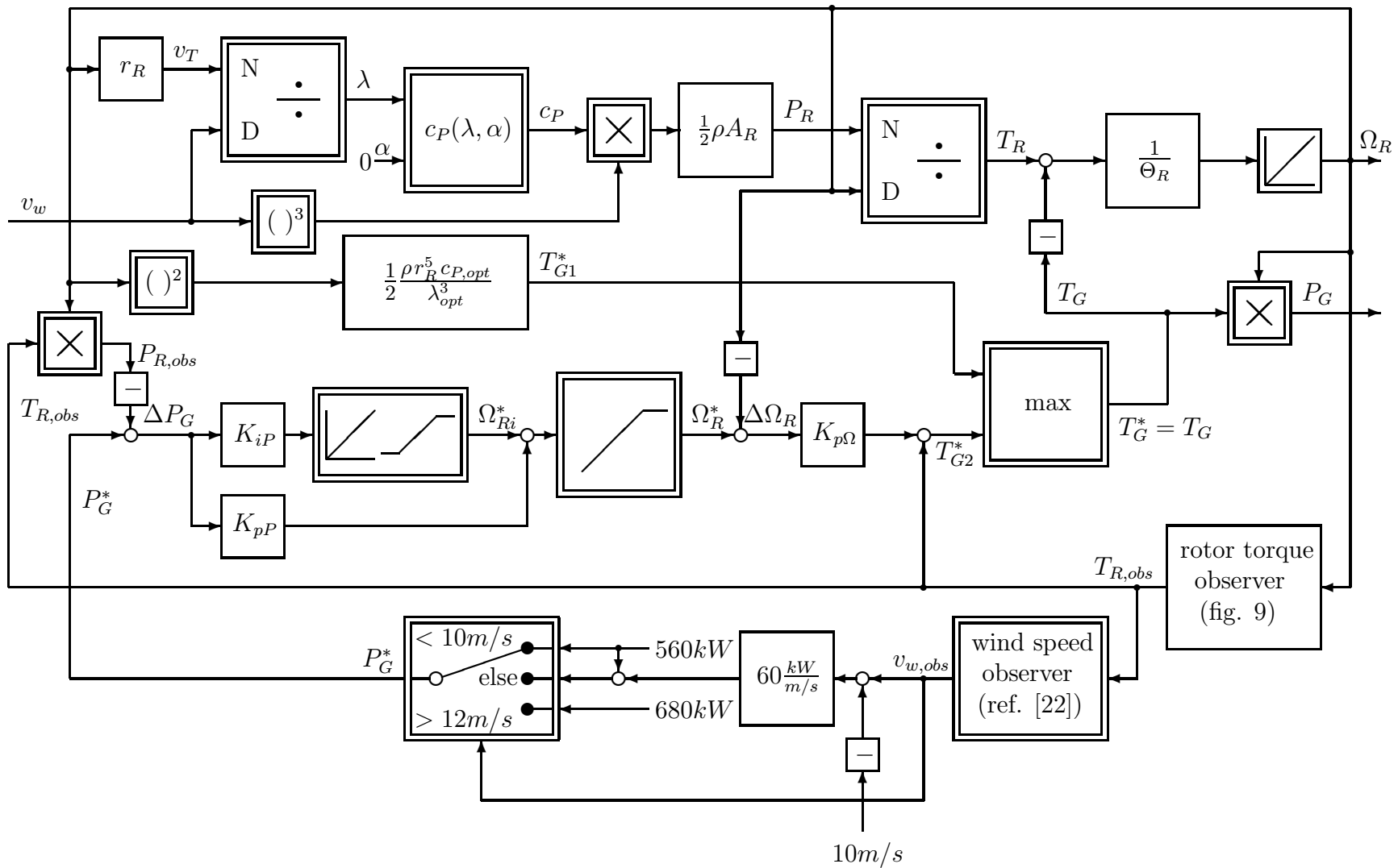
Figure 62: The stall controlled variable speed concept. Important note: The wind speed observer has not been used in the simulations! Instead, the actual wind speed v_w was used as observed wind speed v_{w,obs} , too, which means that the behaviour of the wind speed observer was assumed to be ideal. The reason for this was to speed up the simulation.
