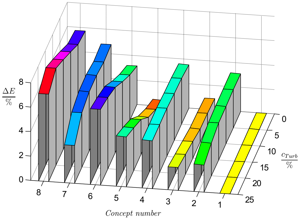
Figure 45: Energy gain of the concepts over concept 1 as a function of c_{Turb} . Parameters: \bar{v}_{w,a} = 7m/s , k = 2 , \lambda_D = 6 , profile Goe 758.
